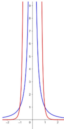
Figure 2: ratio of derivative of gravitational force and the force (y-axis) depending on the distance between the observer and the object (x-axis) for 3-dimensional space (blue) and 9-dimensional space (red)
